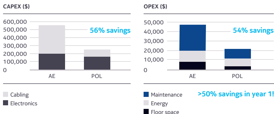
POL vs Ethernet LAN: cost comparison for 2,000 end-points over 10 floors
